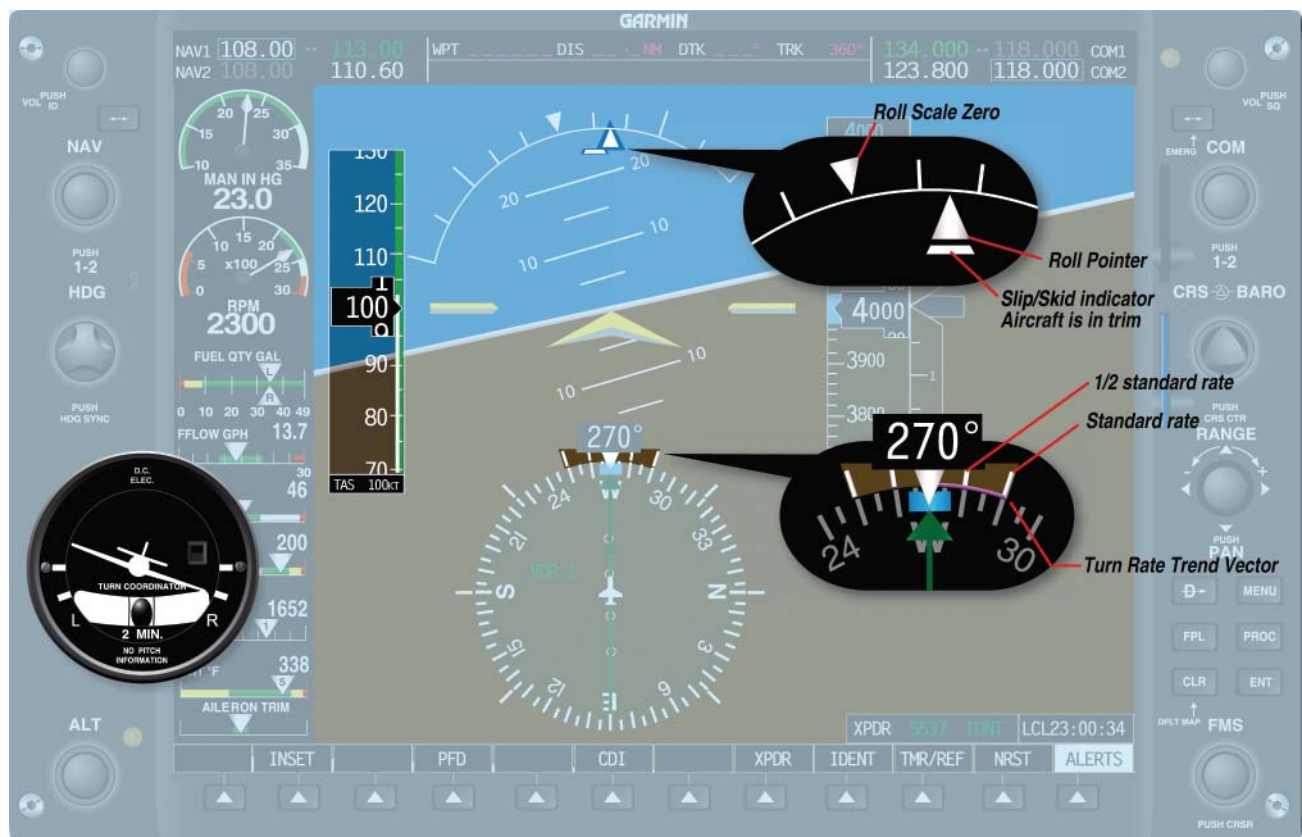
Figure 4-32. Primary Bank.
