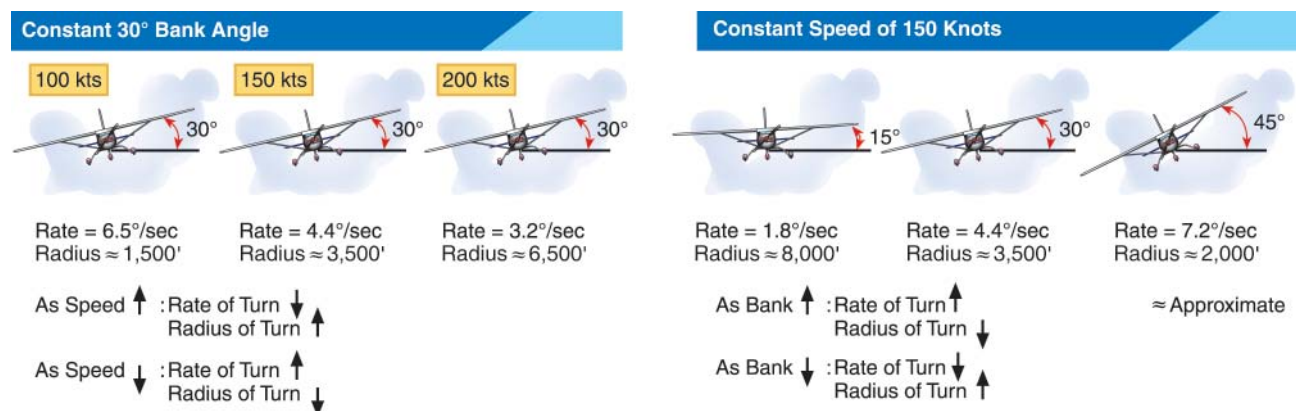
Figure 2-14. Turns.
