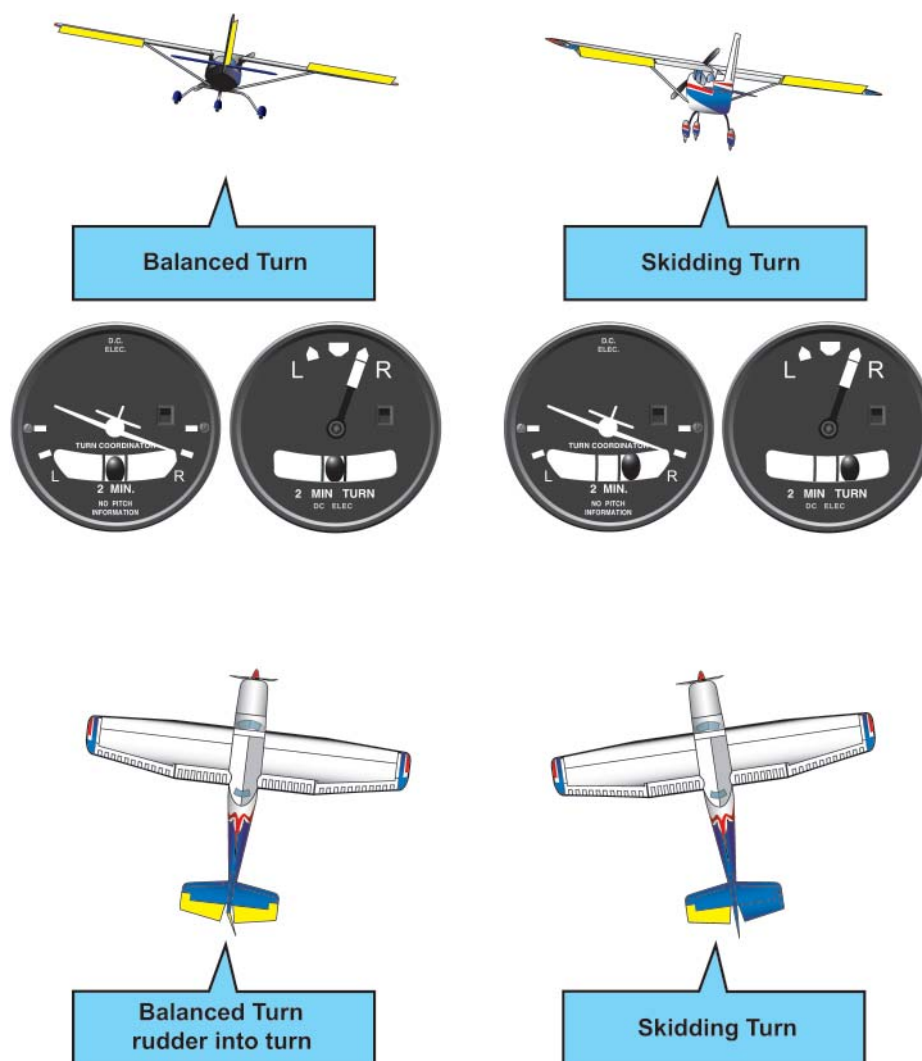
Figure 2-15. Adverse Yaw.
