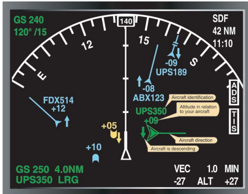
Figure 3-49. An aircraft equipped with ADS will receive identification, altitude in hundreds of feet (above or below using + or -), direction of the traffic, and aircraft descent or climb using an up or down arrow. The yellow target is an illustration of how a non-ADS equipped aircraft would appear on an ADS-equipped aircraft's display.
