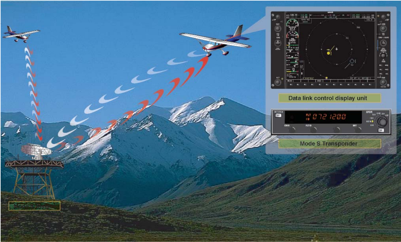
Figure 3-54. Concept of the Traffic Information System.
