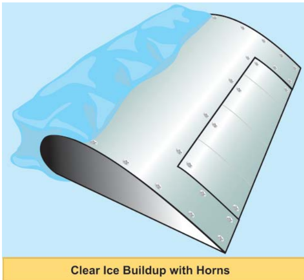
Figure 2-17. Clear Ice Buildup.
