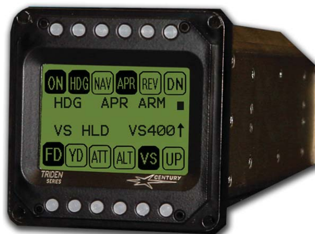
Figure 3-42. An Autopilot by Century.
