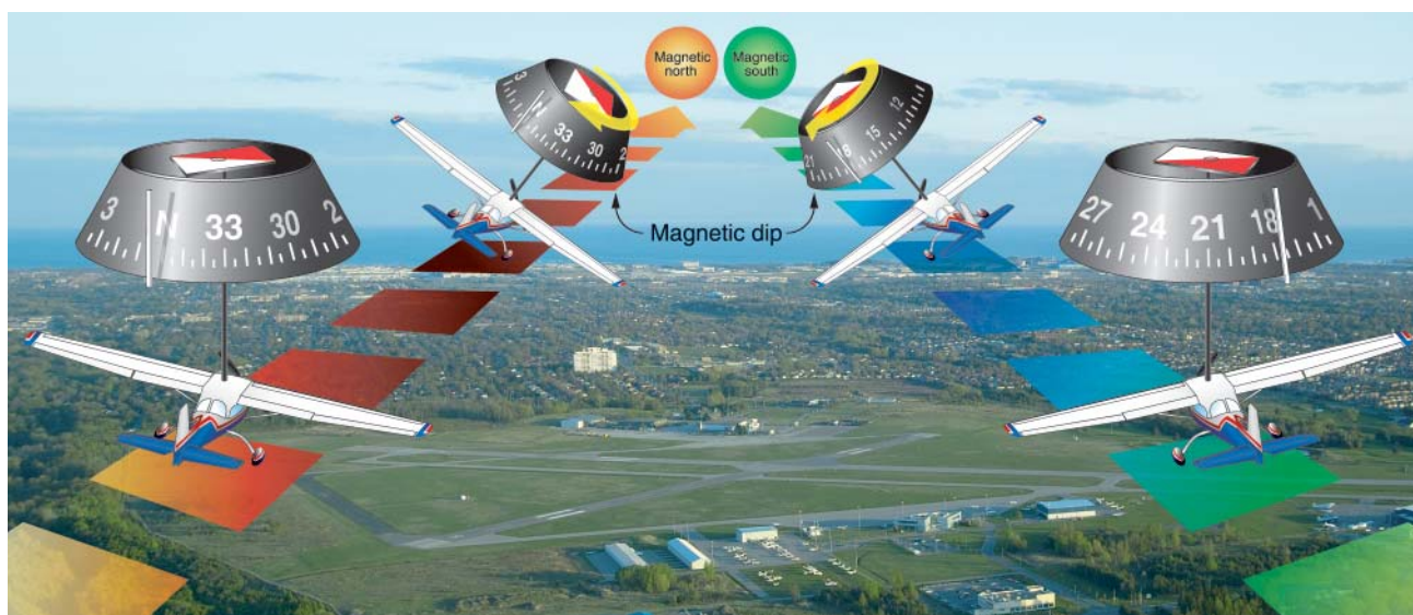
Figure 3-20. Northerly Turning Error.
